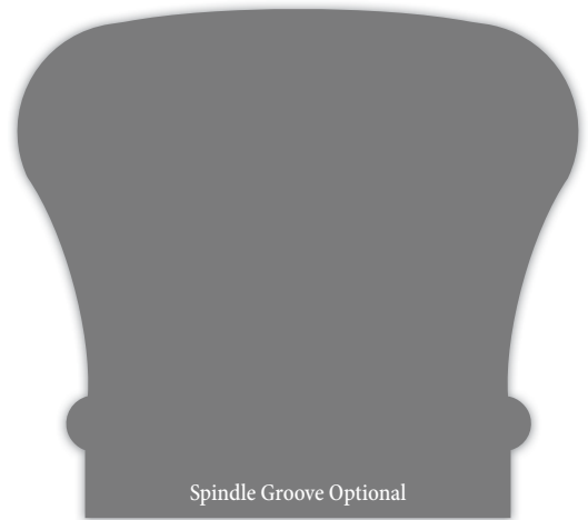
HWP4059 Handrail 2.375"x 2.625"
