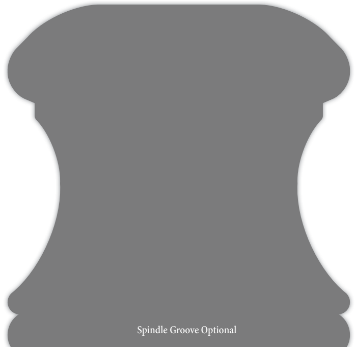
HWP4563 Handrail 3.500"x 3.500"
