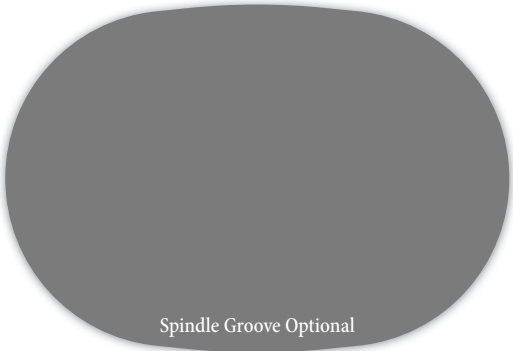
HWP4054 Handrail 1.562"x 1.812"
