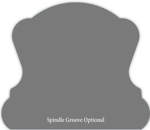
HWP4255 Handrail 2.250"x 2.625"
