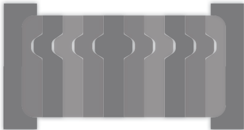
HWP4008B Handrail 1.062" X 2.125"
