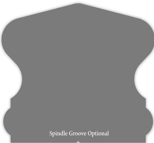
HWP4596 Handrail 2.375"x 2.625"
