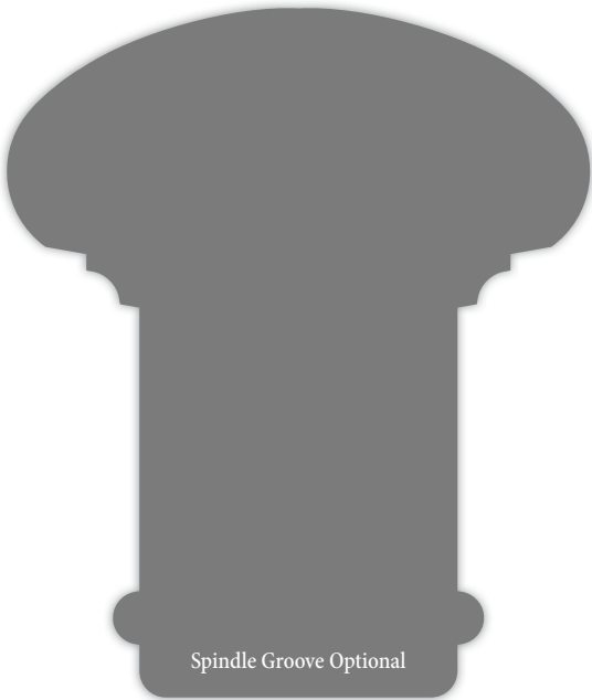
HWP4551 Handrail 3.250"x 2.750"
