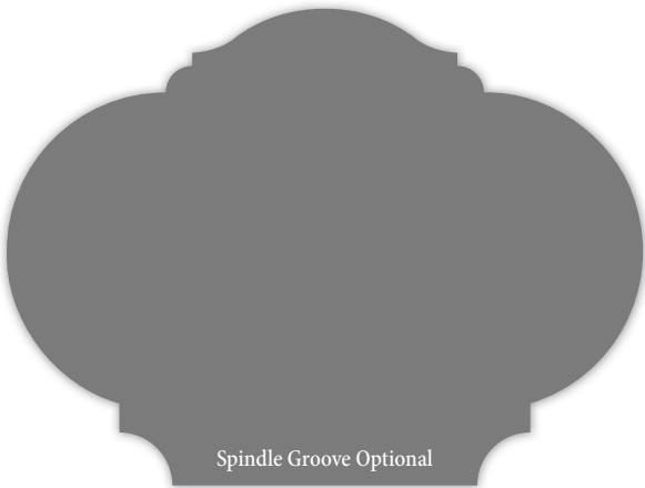
HWP4553 Handrail 2.250"x 3.000"
