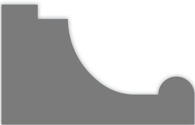
HWP7244 Molding 1.250"x 2.000"
