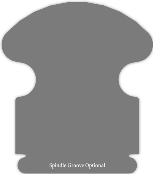
HWP4250 Handrail 3.125"x 2.750"
