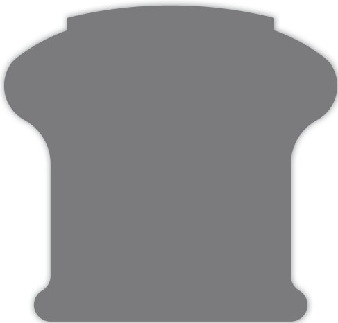
HWP4001 Handrail 2.375" x 2.500"
