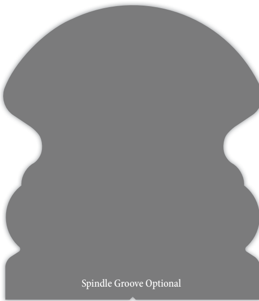
HWP4594 Handrail 3.000"x 2.625"
