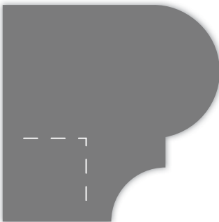
HWP4585 Nosing 1.625"x 1.625"
