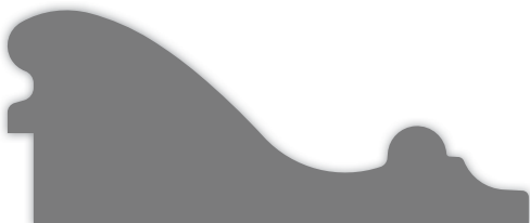
HWP8559 Panel Mold 1.032"x 2.500"
