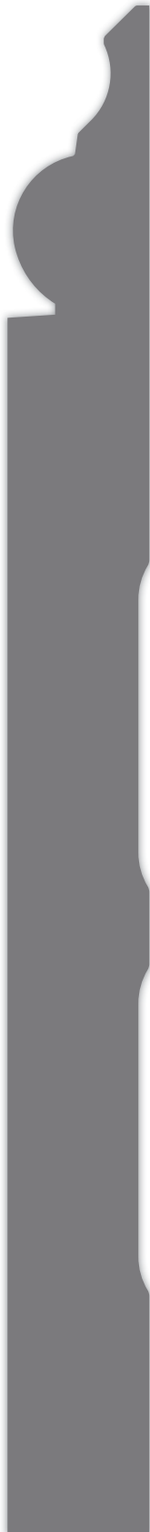
HWP3508 Base 0.812" x Variable
